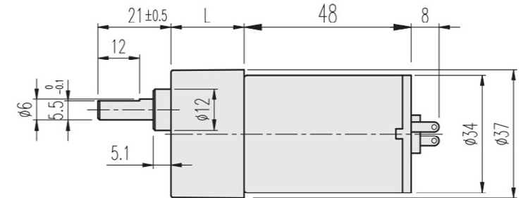
GEARHEAD LENGTH
